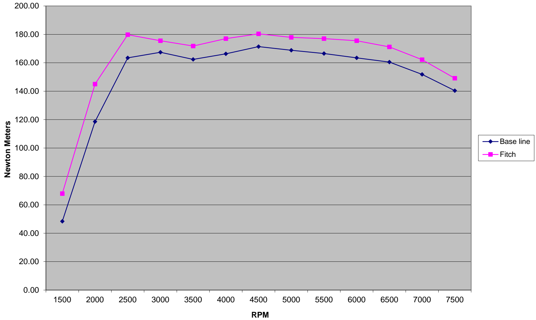
2008 Ford Focus Torque Data Dastek Data
